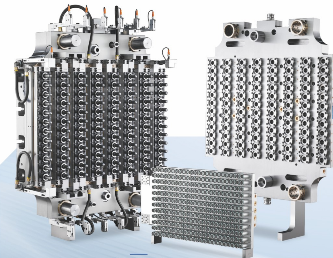
96 腔注坯系统模具 96 Cavity Injection System Mould Adapted To HUSKY HyPET400
