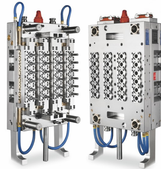
24腔化妆品瓶坯模具 24 Cavities Cosmetic Preform Mould
