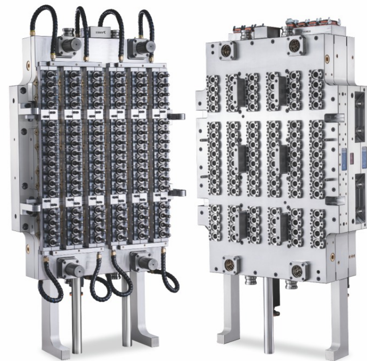
96 Cavity Preform Mould 96 腔瓶坯模具
