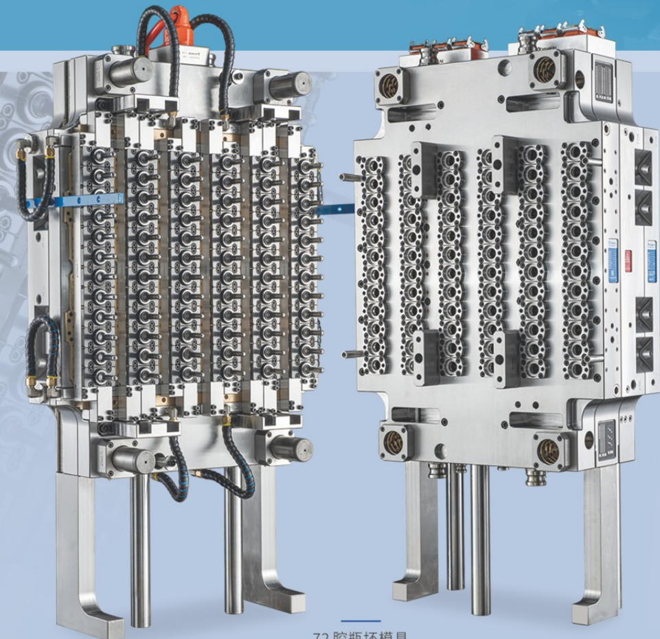
72腔瓶坯模具 72 Cavities Preform Mould
