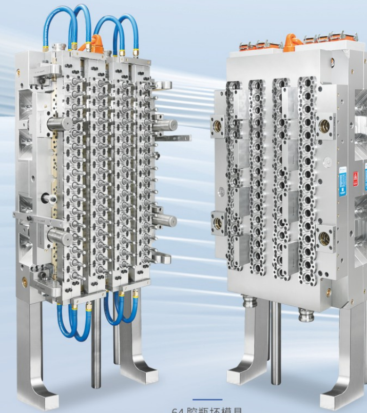
64腔瓶坯模具 64 Cavities Preform Mould
