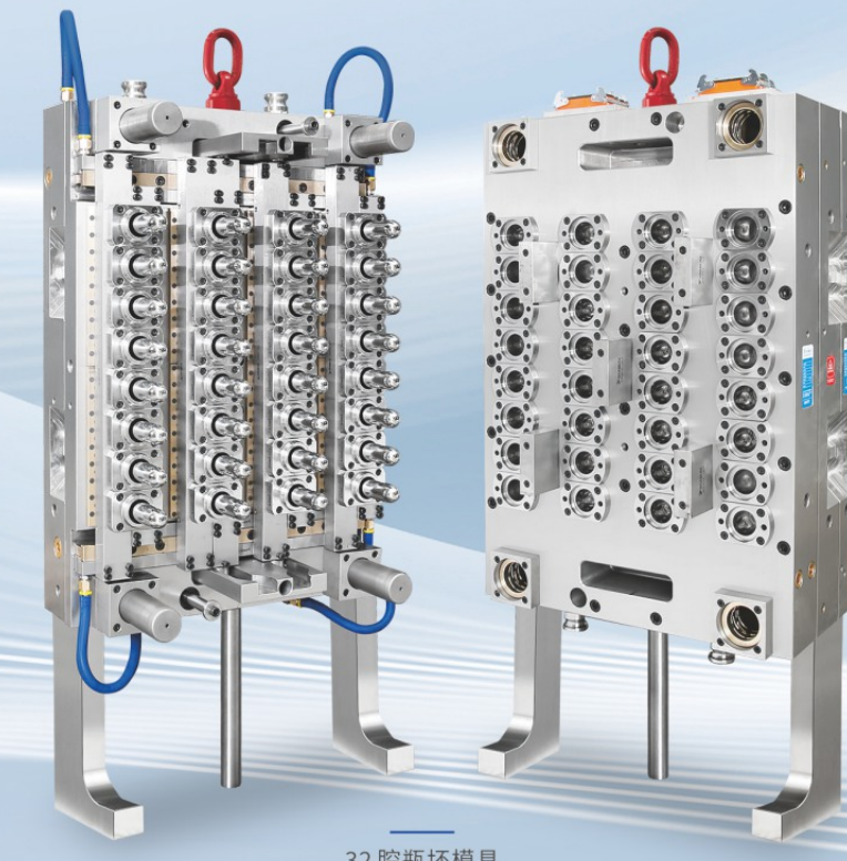
32腔瓶坯模具 32 Cavities Preform Mould
