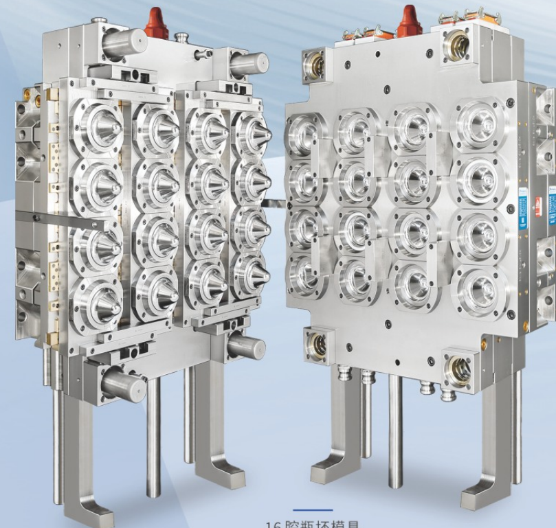
16腔瓶坯模具 16 Cavities Preform Mould
